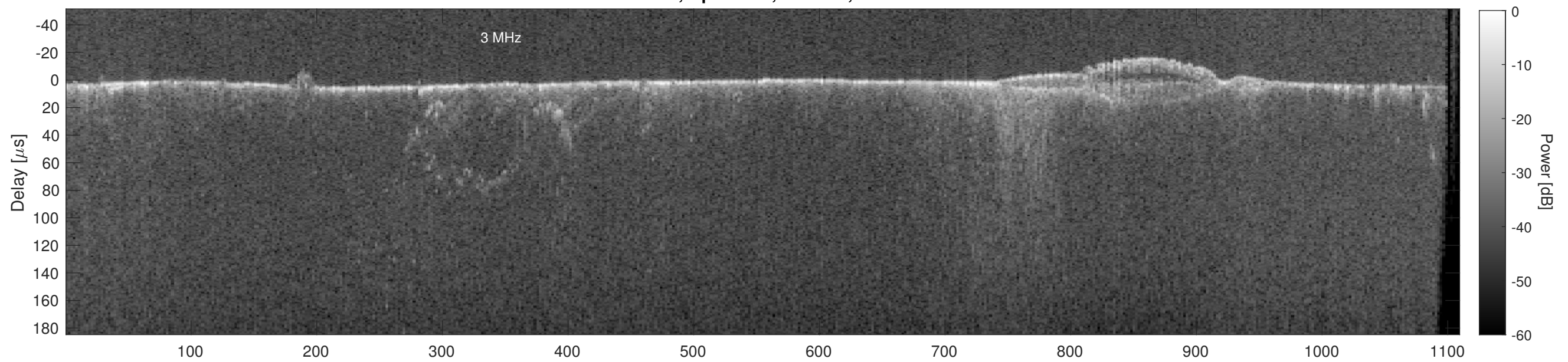
Orbit 14126, Cluttergram
