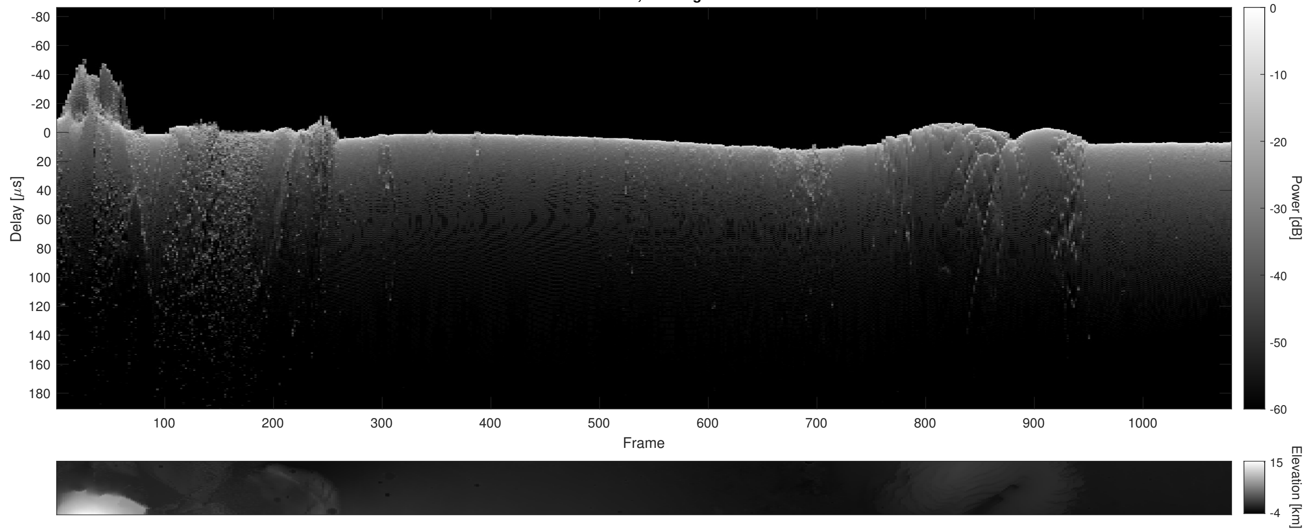
Orbit 14129, Cluttergram
