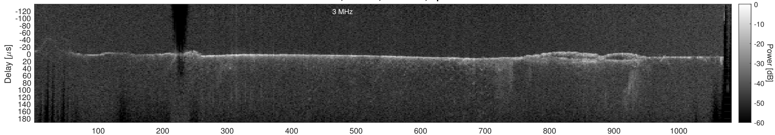
Orbit 14129, Cluttergram
