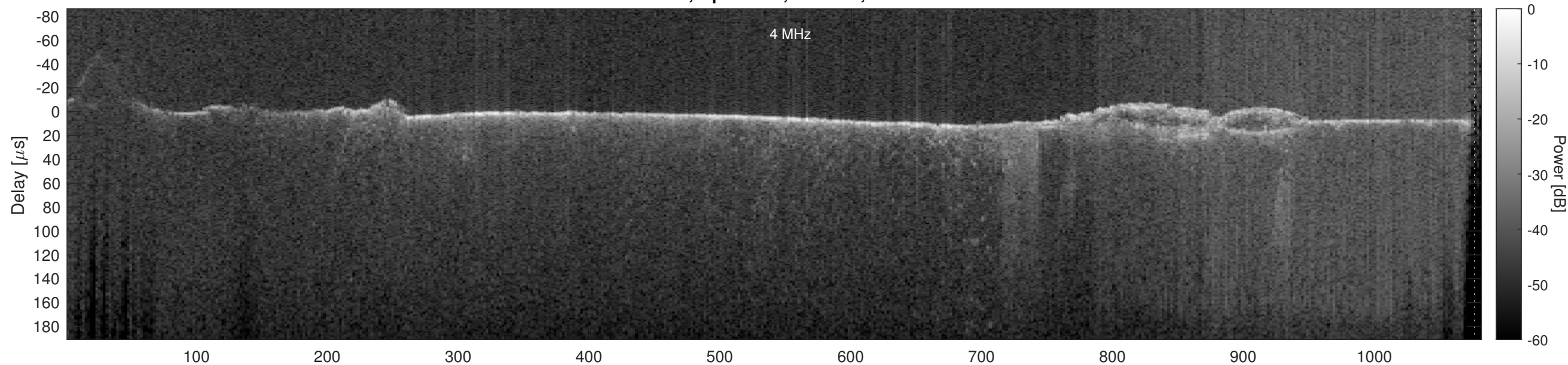
Orbit 14129, Optimized, Window, Channel 2
