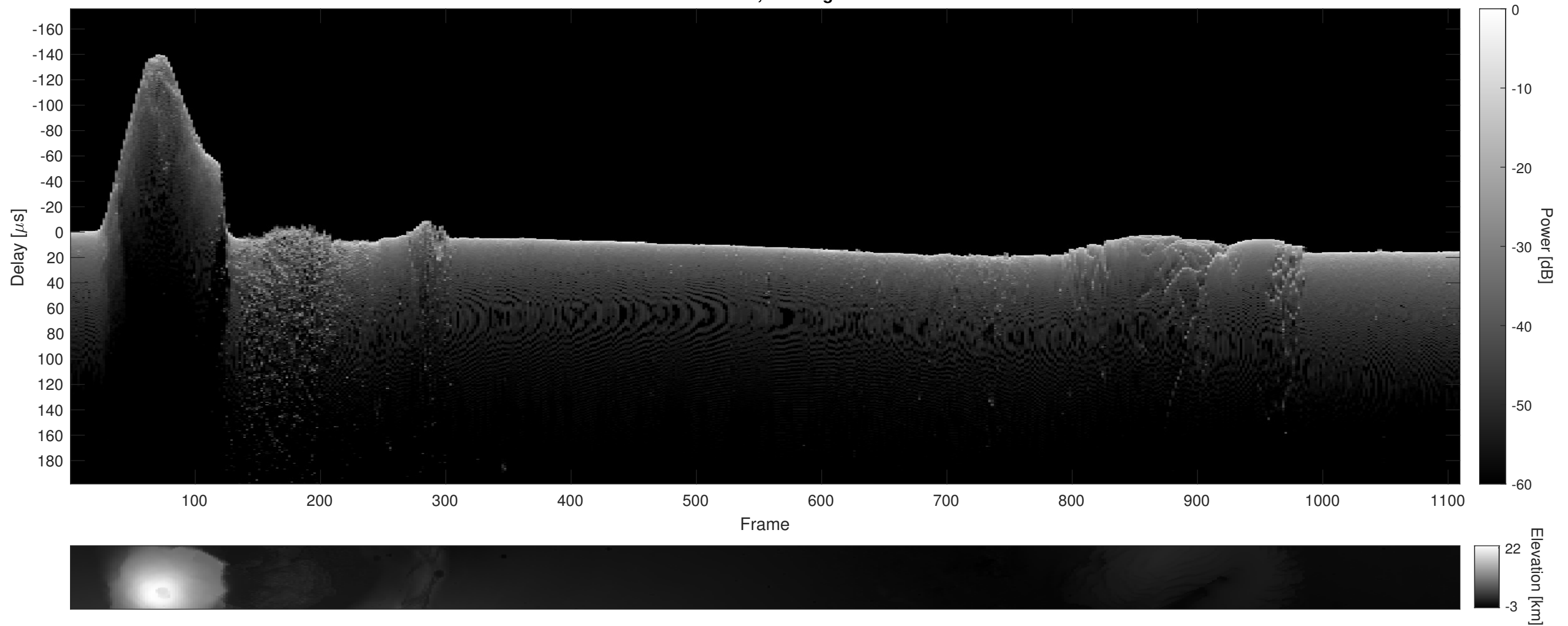
Orbit 14136, Cluttergram
