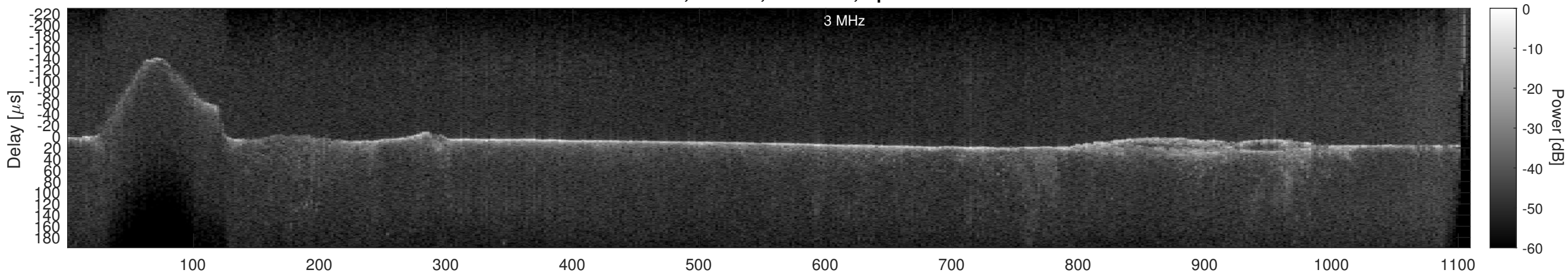
Orbit 14136, Cluttergram
