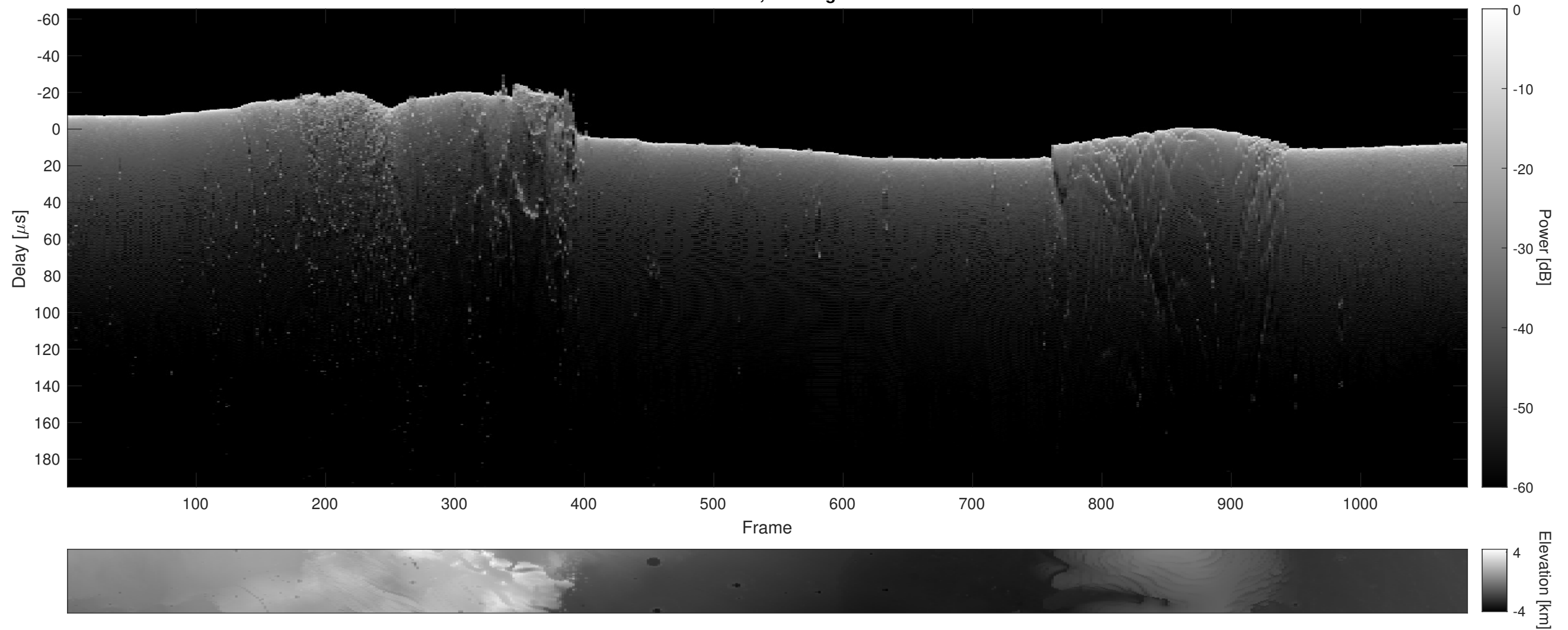
Orbit 14139, Cluttergram
