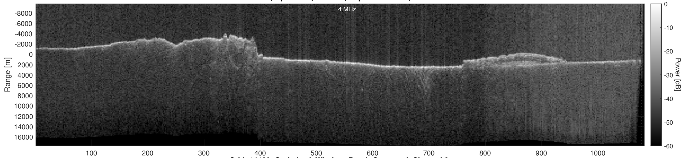
Orbit 14139, Optimized, Window, Depth-Corrected, Channel 2
