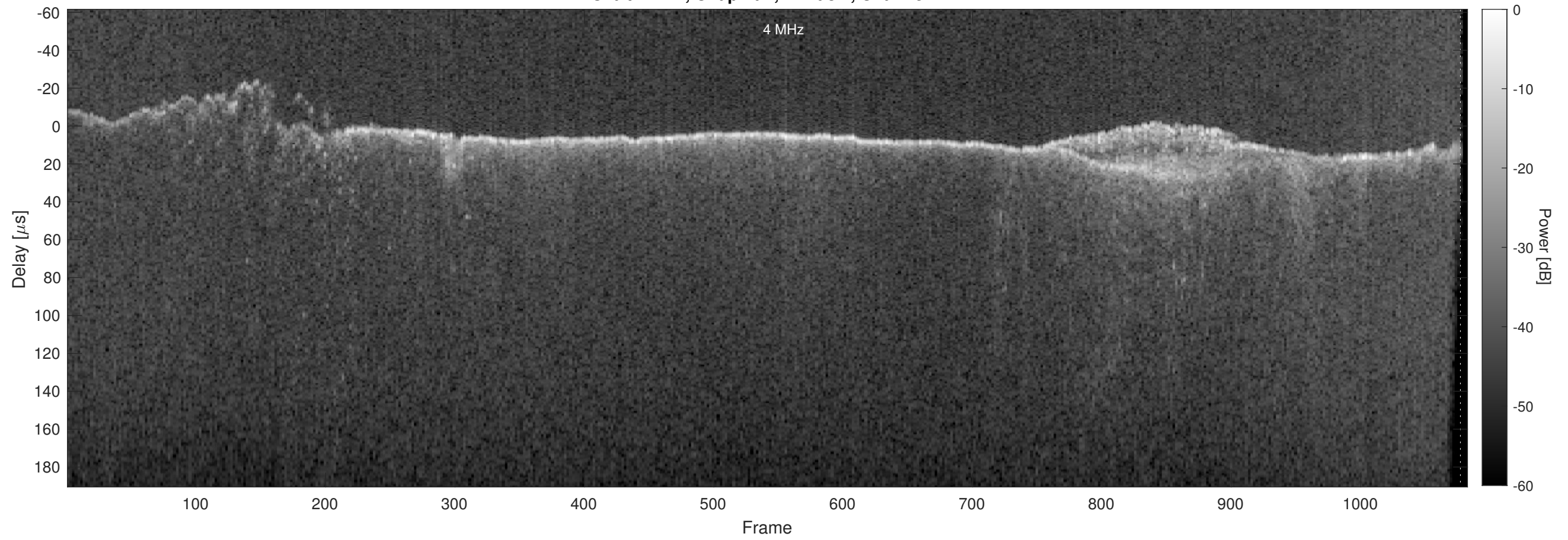
Orbit 14141, Chapman, Window, Channel 2
