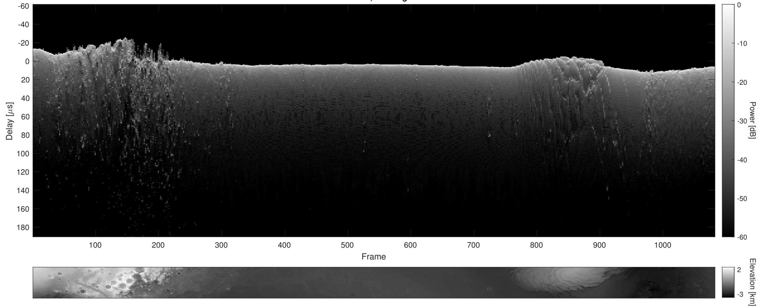
Orbit 14141, Cluttergram
