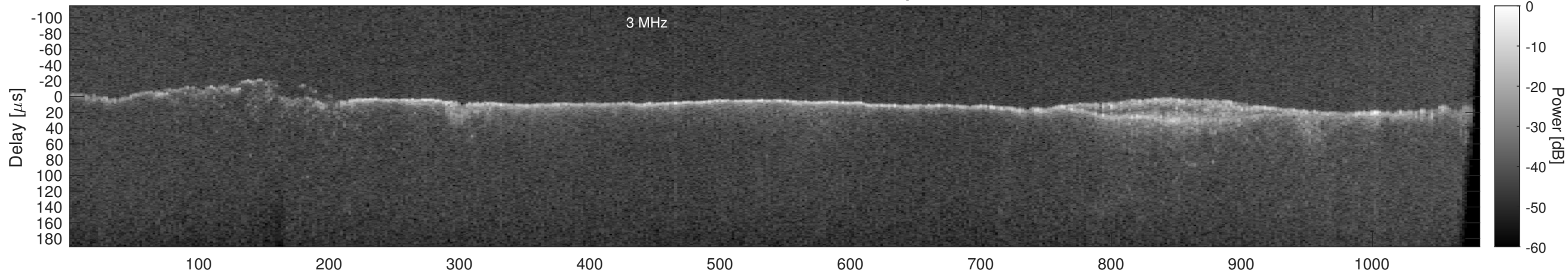
Orbit 14141, Window, Channel 2, Optimized
