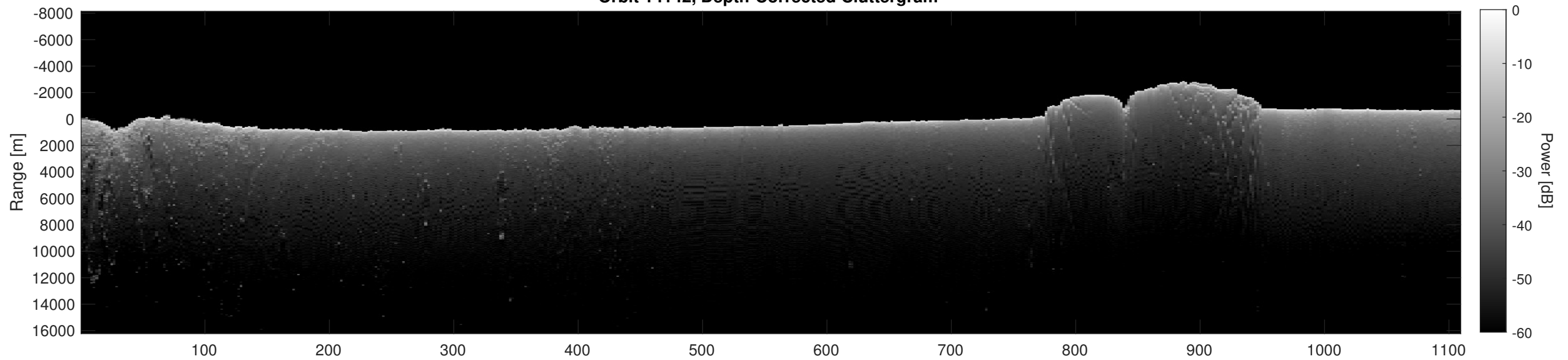
Orbit 14142, Depth-Corrected Cluttergram
