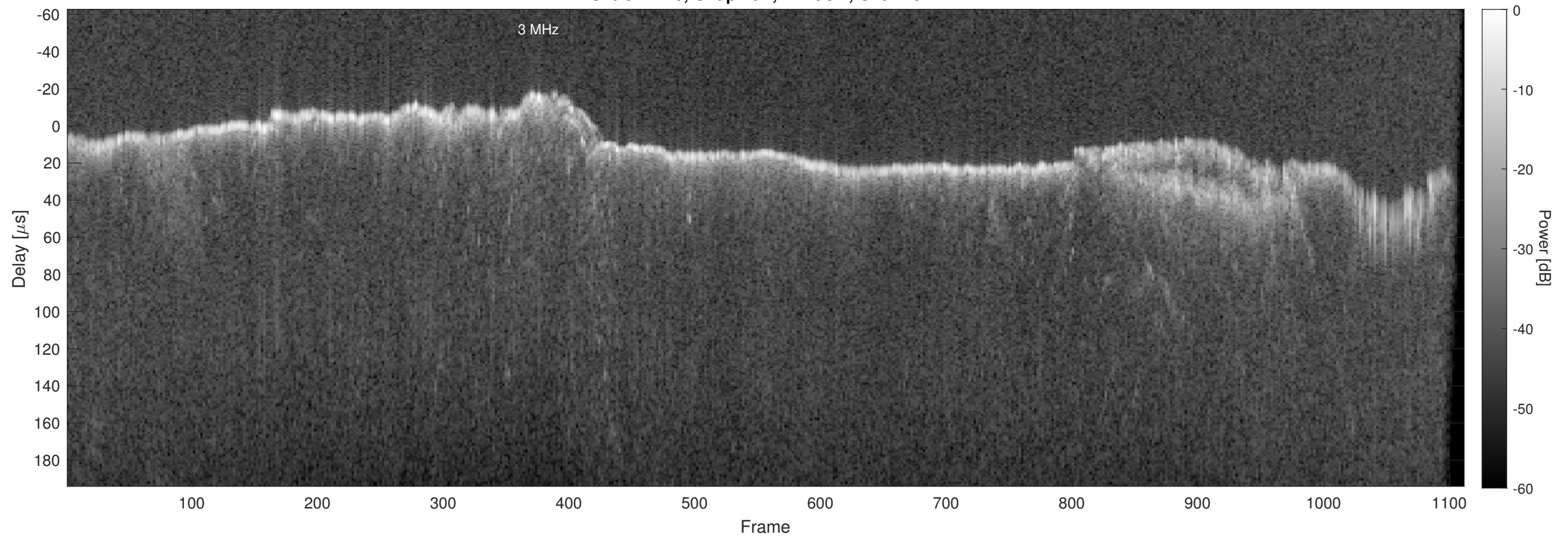
Orbit 14146, Chapman, Window, Channel 2
