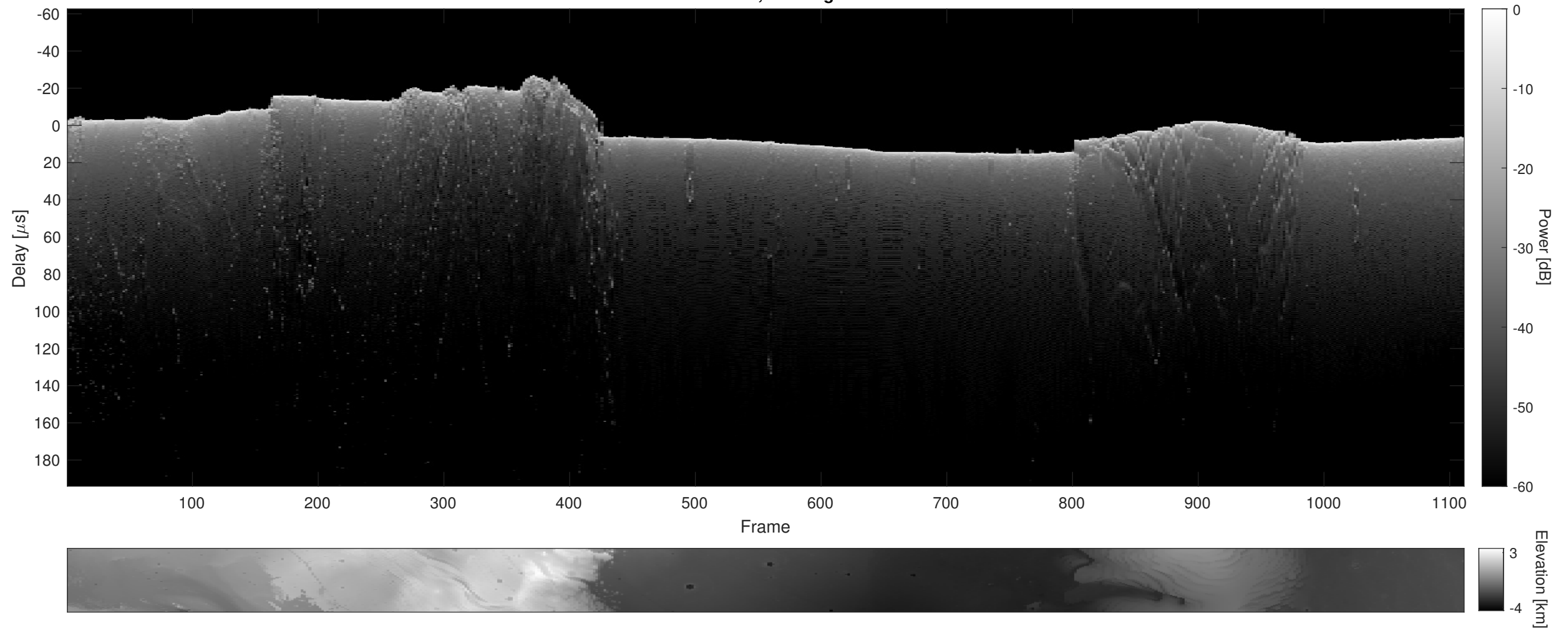
Orbit 14146, Cluttergram
