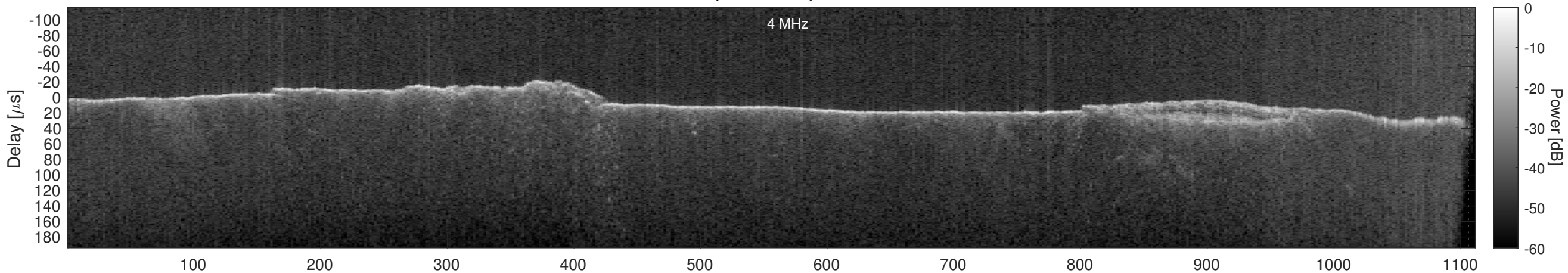
Orbit 14146, Window, Channel 1, Chapman
