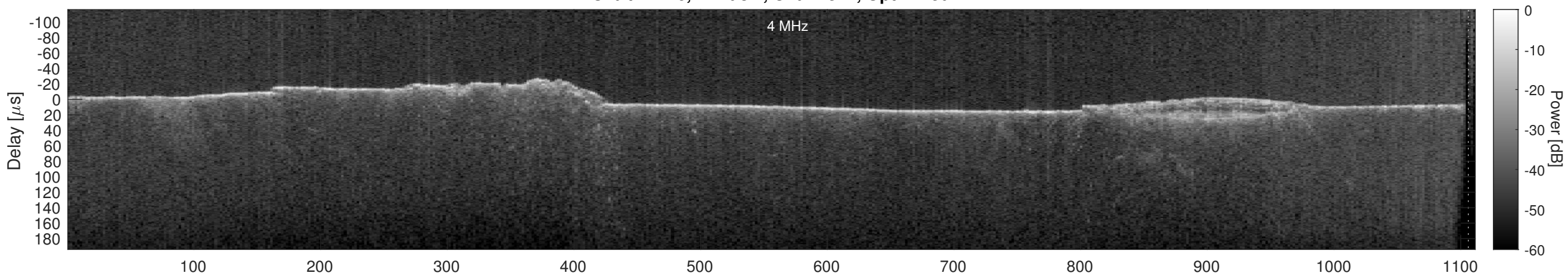
Orbit 14146, Cluttergram
