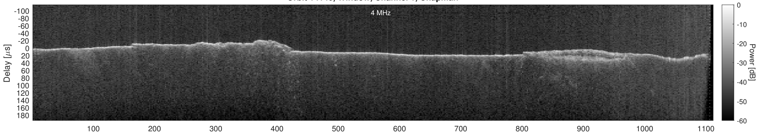
Orbit 14146, Window, Channel 1, Optimized
