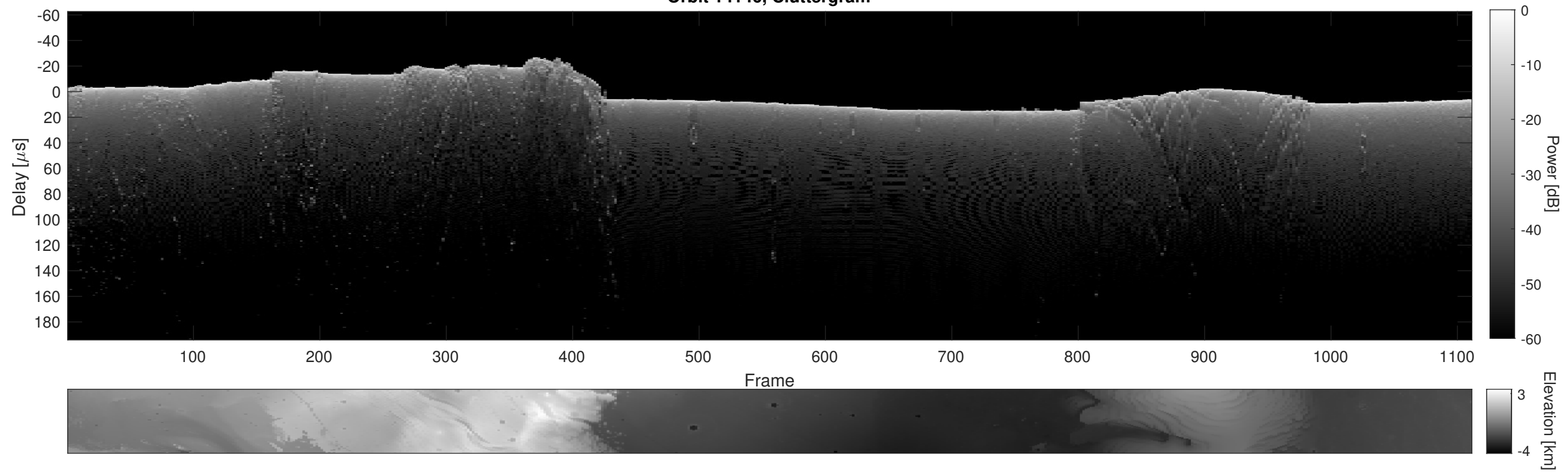
Orbit 14146, Cluttergram
