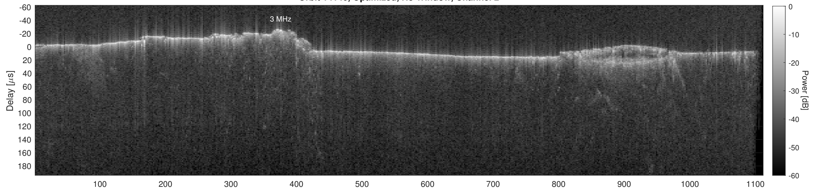
Orbit 14146, Cluttergram
