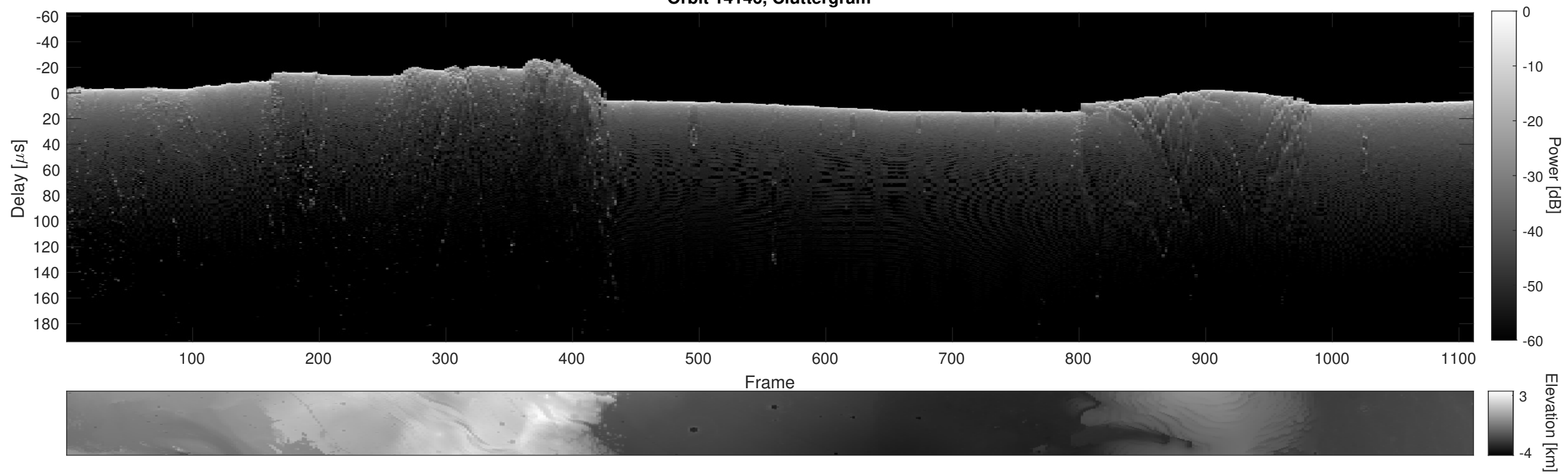
Orbit 14146, Cluttergram
