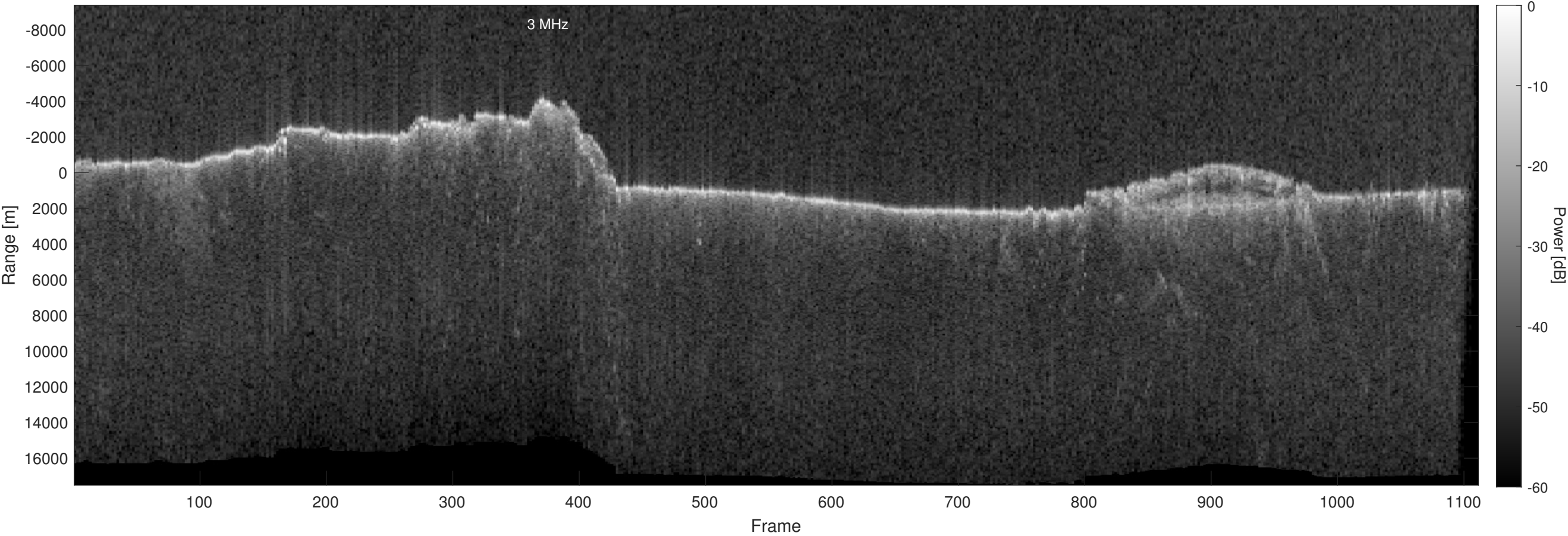
Orbit 14146, Optimized, Window, Depth-Corrected, Channel 2
