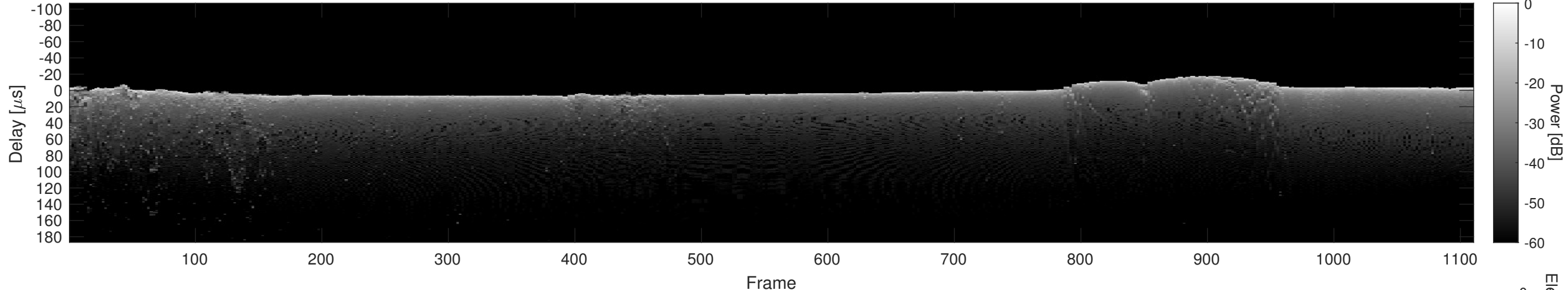
Orbit 14149, Cluttergram
