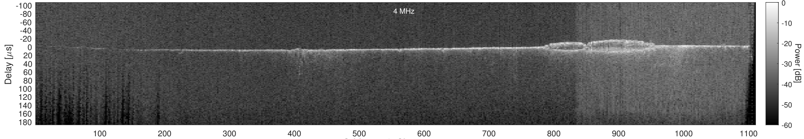
Orbit 14149, Cluttergram
