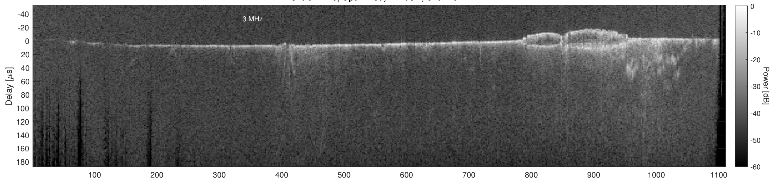
Orbit 14149, Cluttergram
