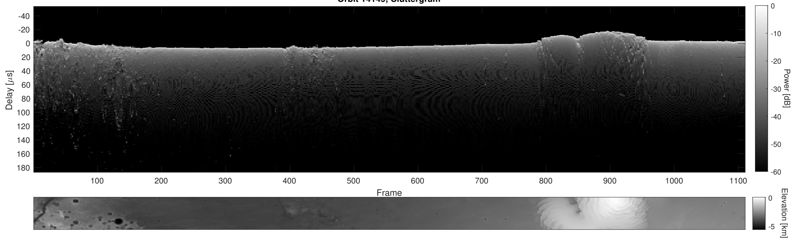
Orbit 14149, Cluttergram
