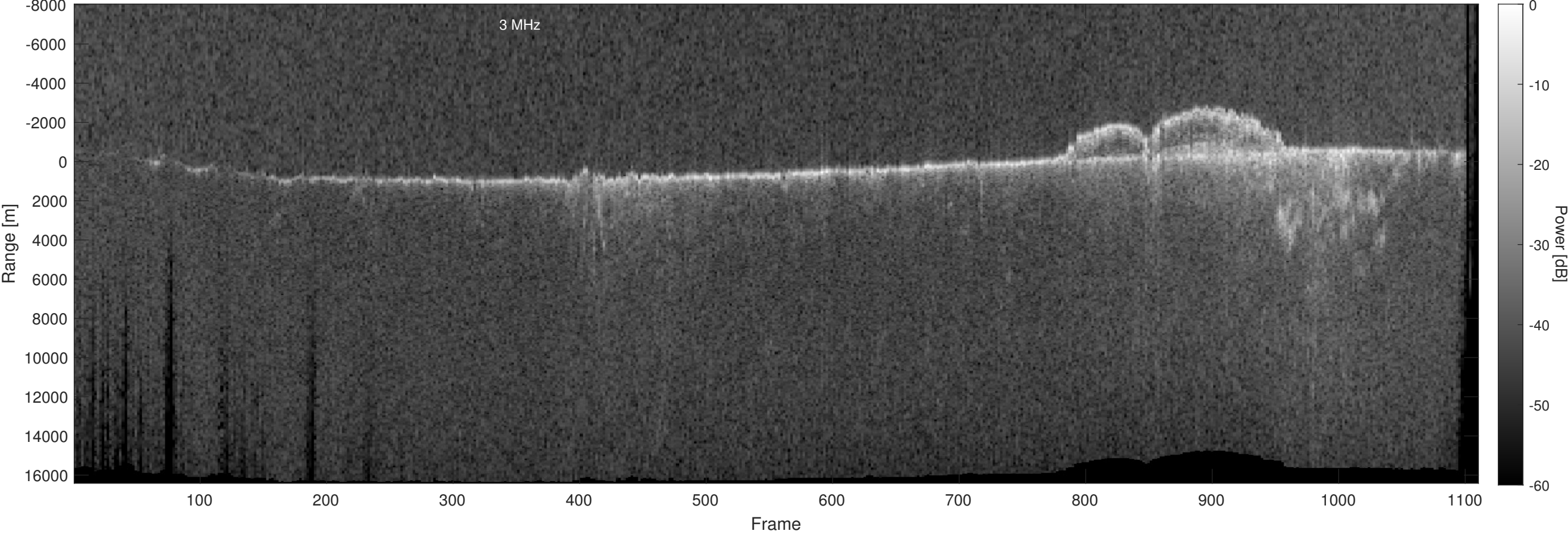
Orbit 14149, Optimized, Window, Depth-Corrected, Channel 2
