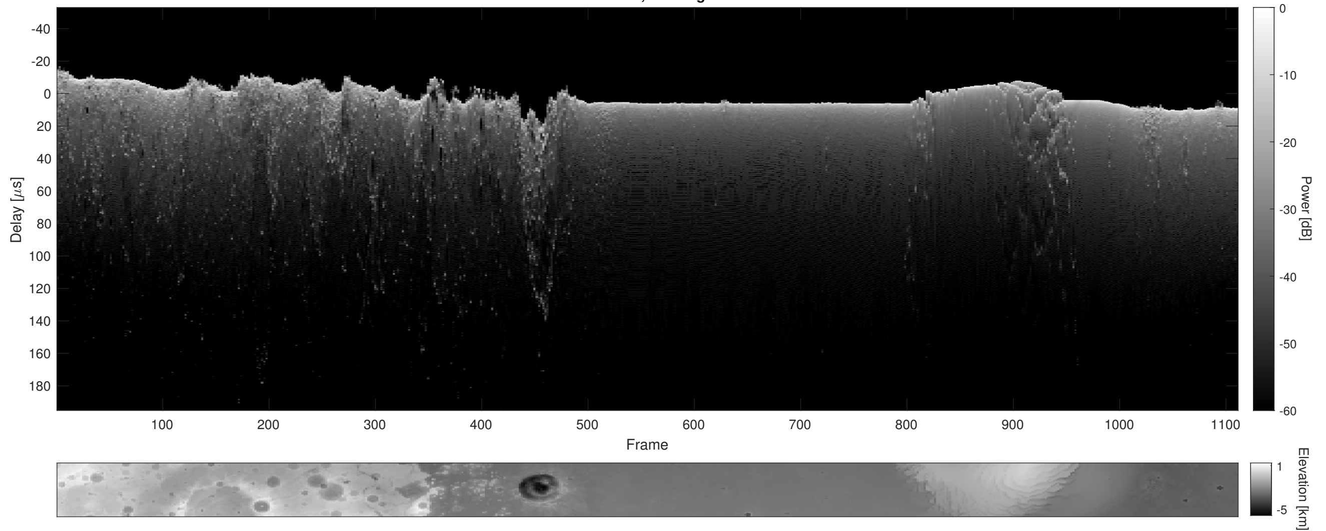
Orbit 14152, Cluttergram
