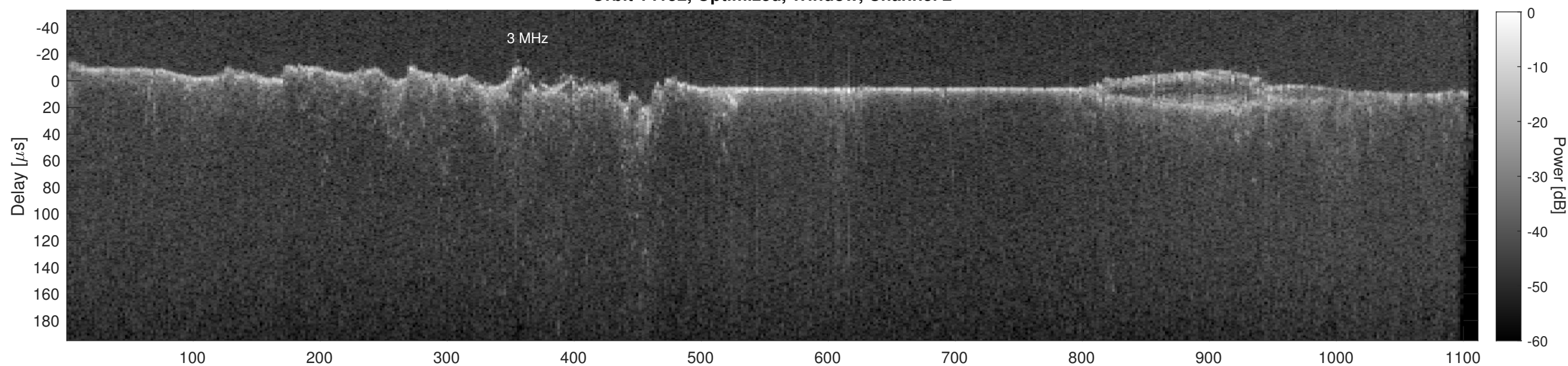
Orbit 14152, Cluttergram
