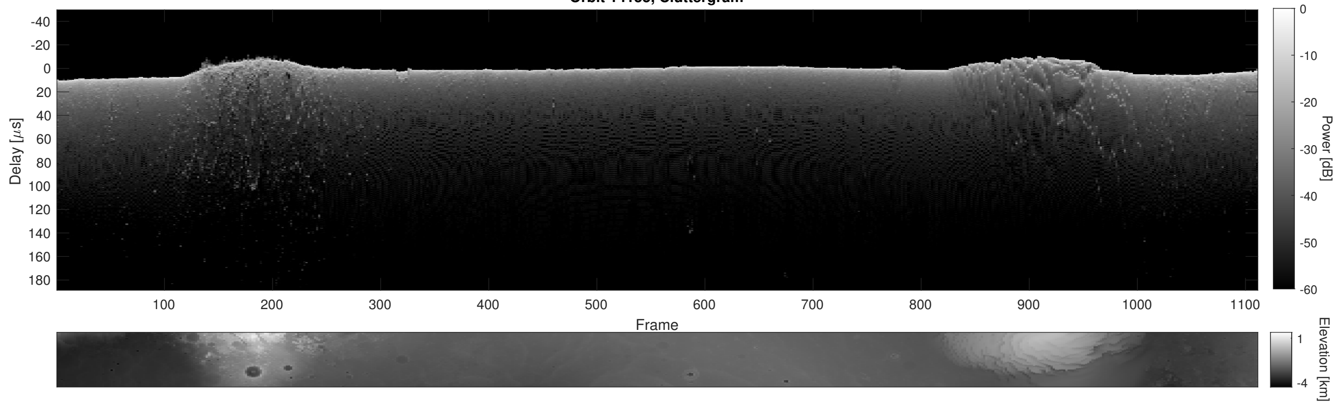
Orbit 14155, Cluttergram
