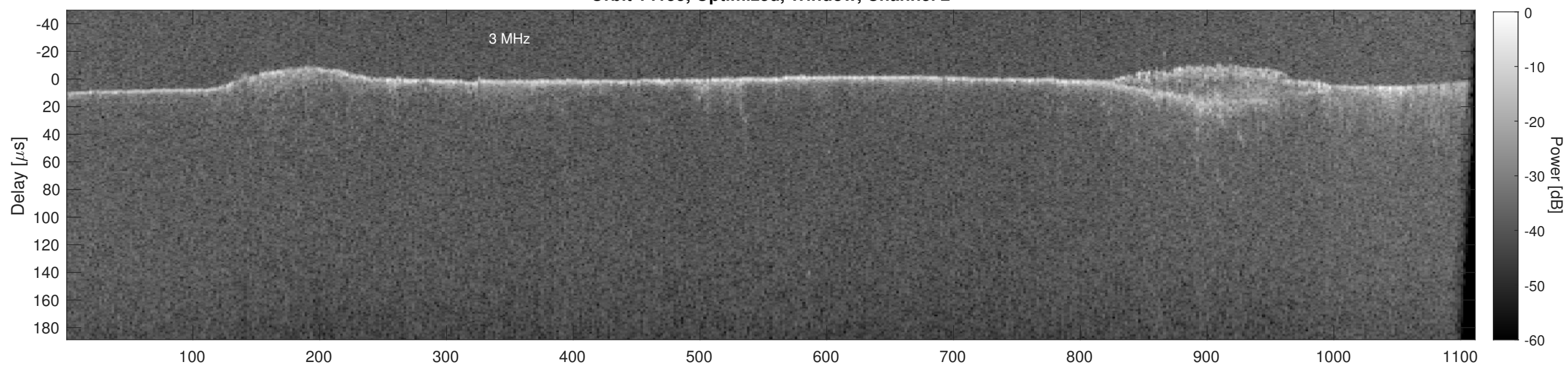
Orbit 14155, Cluttergram
