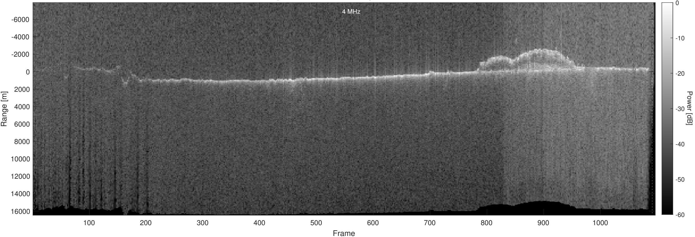
Orbit 14156, Optimized, No Window, Depth-Corrected, Channel 2
