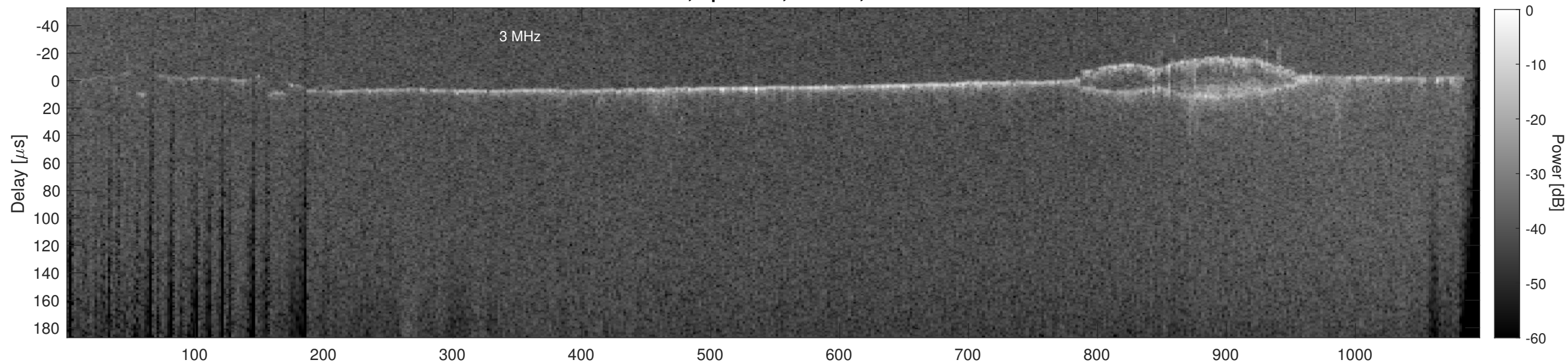
Orbit 14156, Cluttergram
