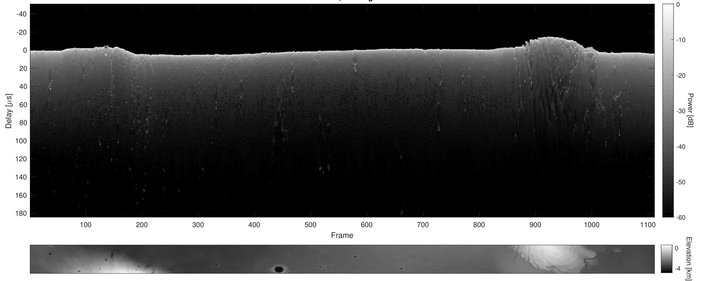
Orbit 14158, Cluttergram
