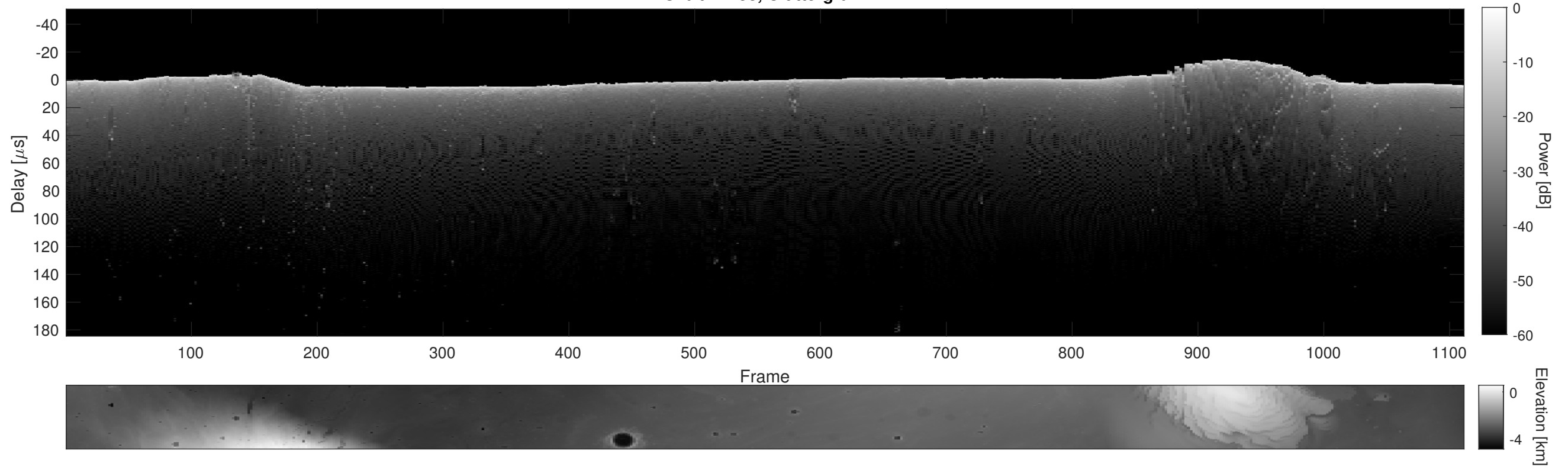
Orbit 14158, Cluttergram
