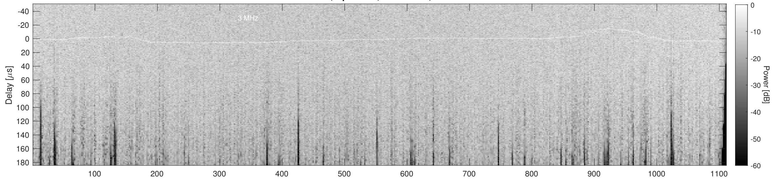
Orbit 14158, Cluttergram
