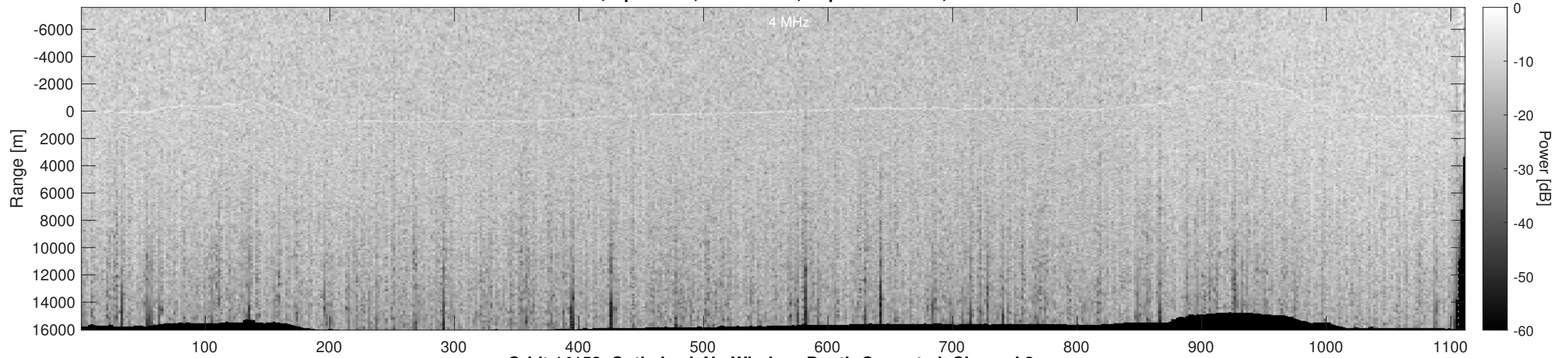
Orbit 14158, Optimized, No Window, Depth-Corrected, Channel 2
