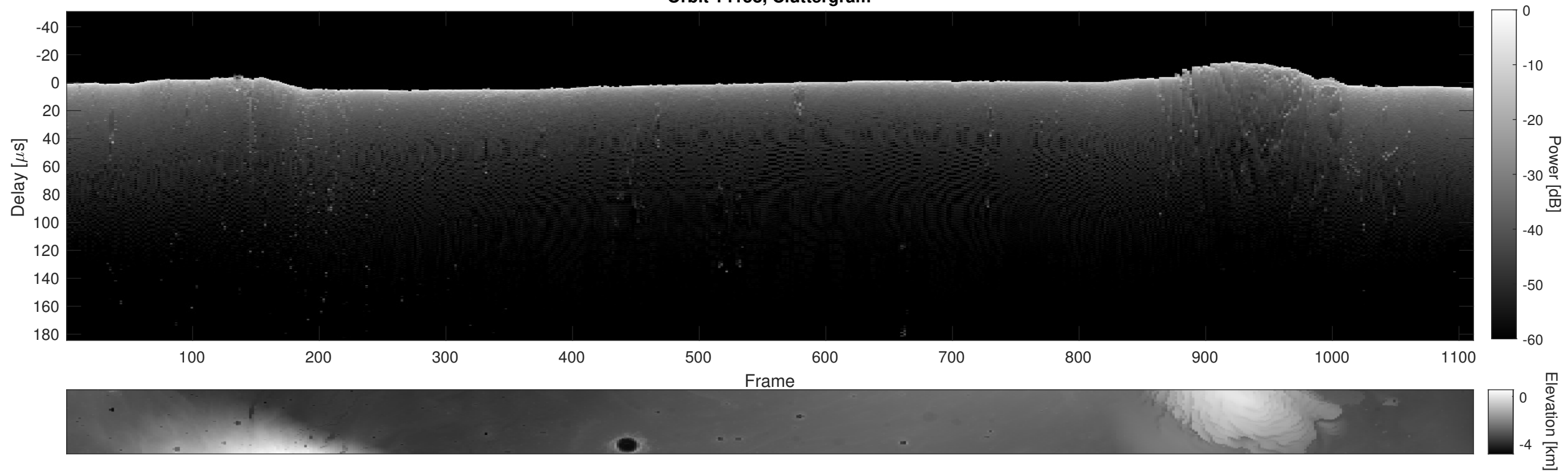
Orbit 14158, Cluttergram
