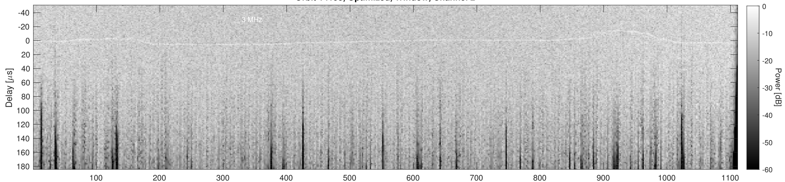
Orbit 14158, Cluttergram
