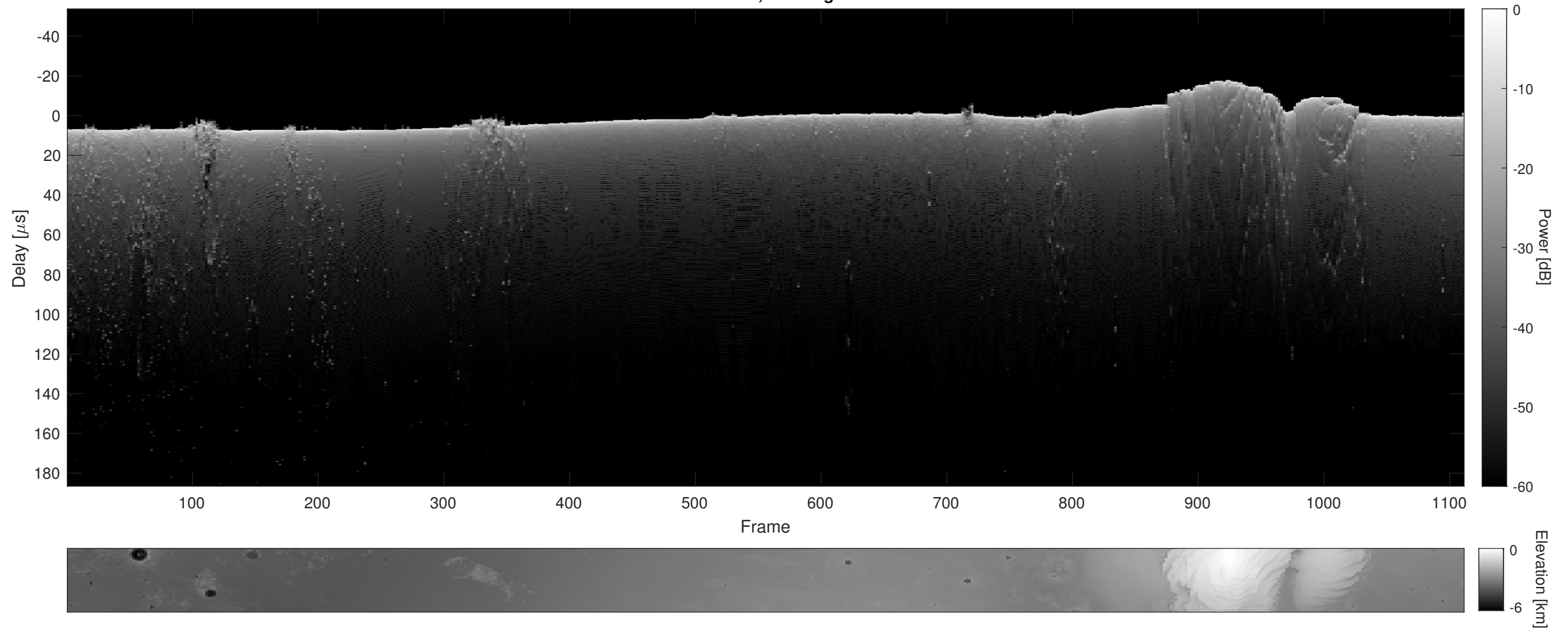
Orbit 14161, Cluttergram
