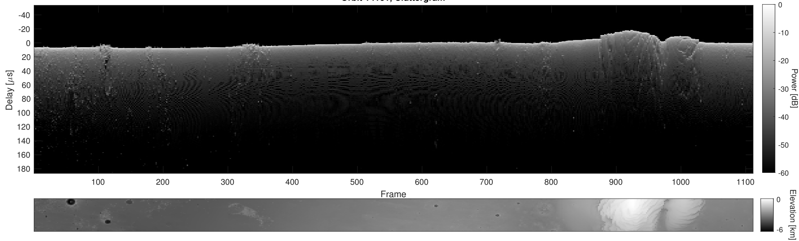
Orbit 14161, Cluttergram
