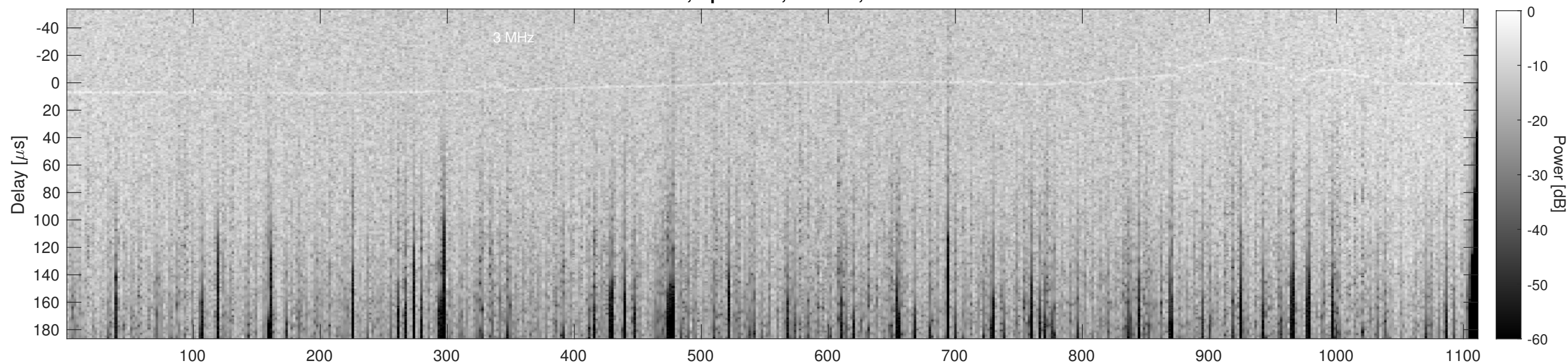
Orbit 14161, Cluttergram
