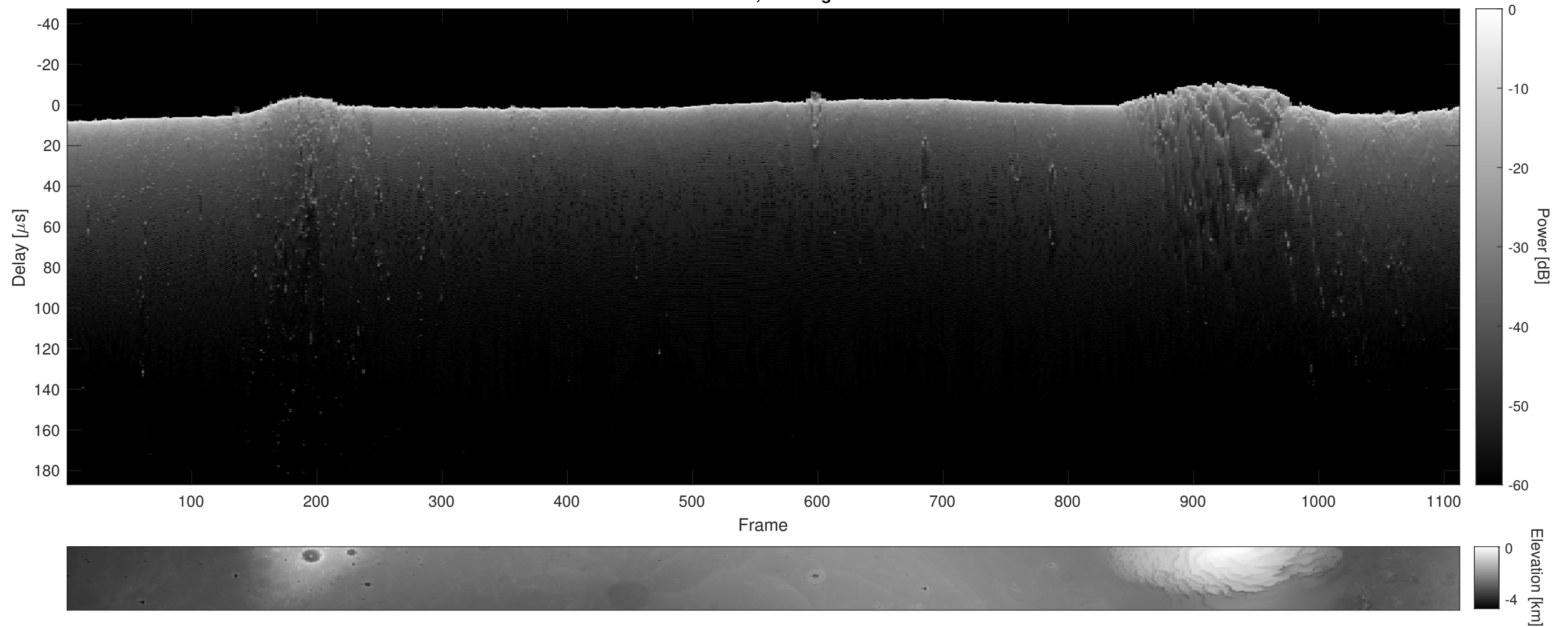
Orbit 14162, Cluttergram
