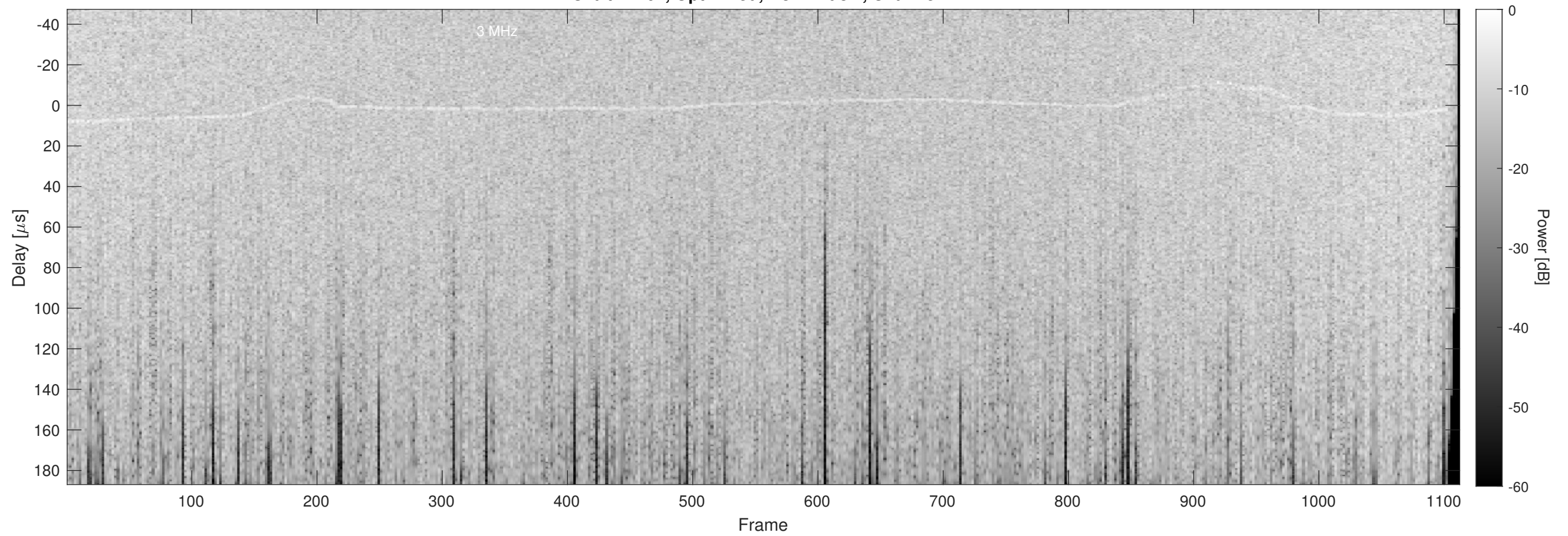
Orbit 14162, Optimized, No Window, Channel 2
