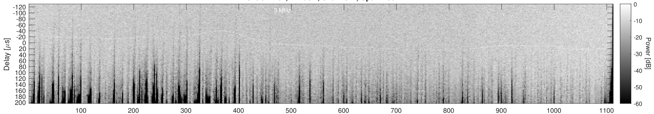
Orbit 14164, Cluttergram
