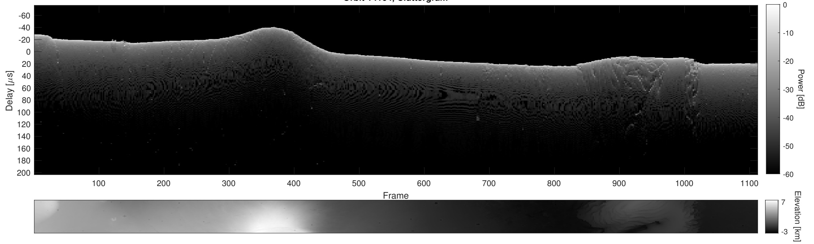
Orbit 14164, Cluttergram
