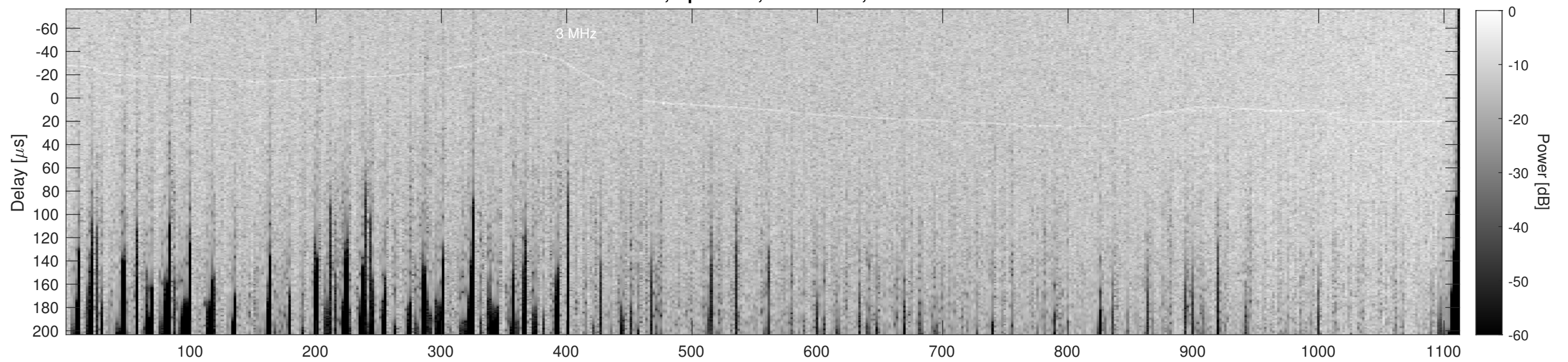
Orbit 14164, Cluttergram
