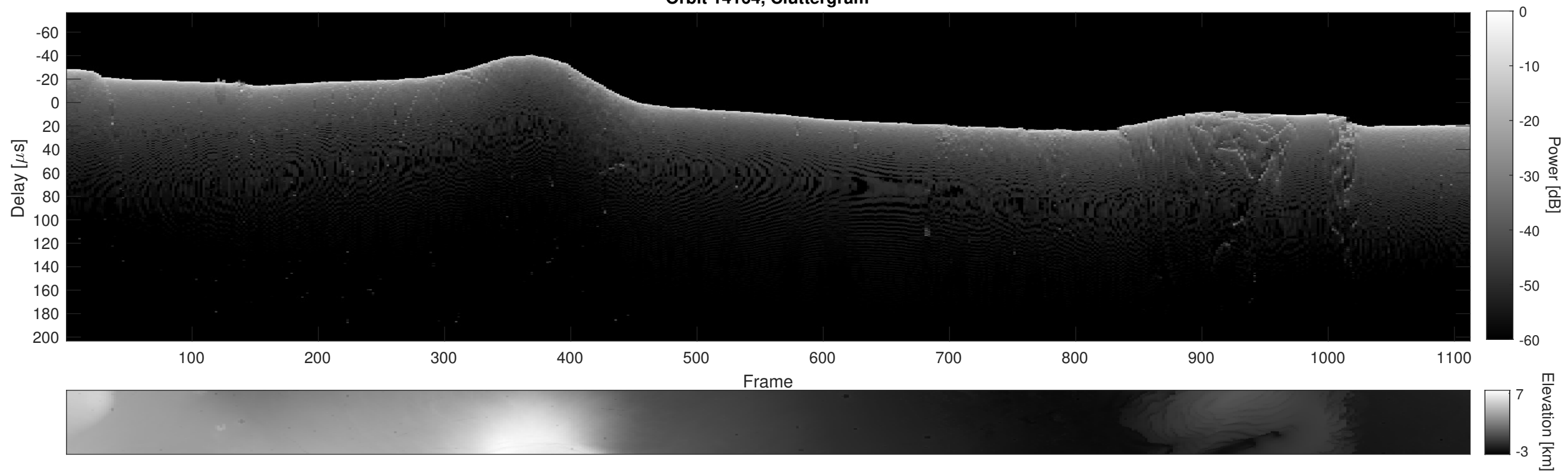
Orbit 14164, Cluttergram
