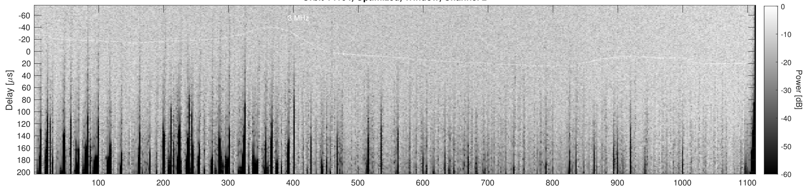
Orbit 14164, Cluttergram
