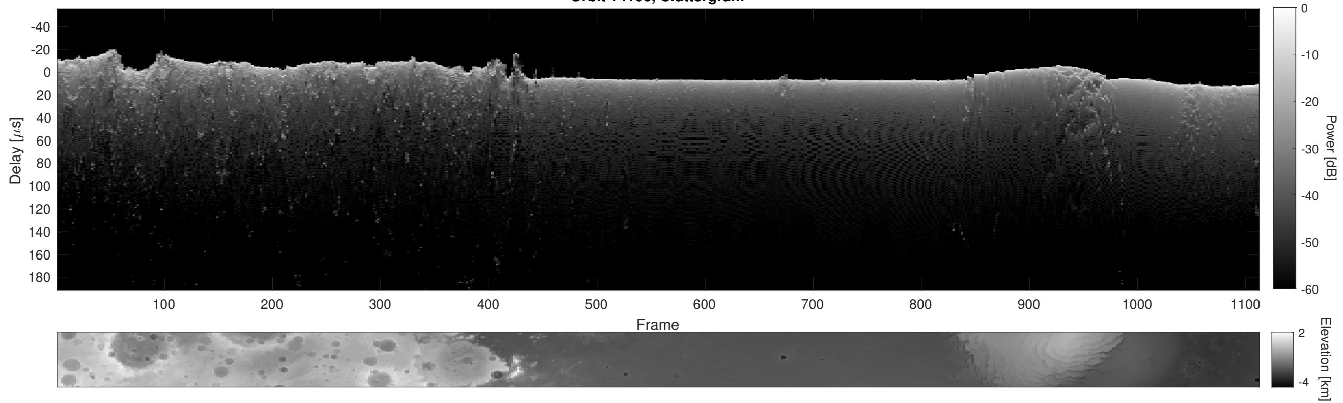
Orbit 14166, Cluttergram
