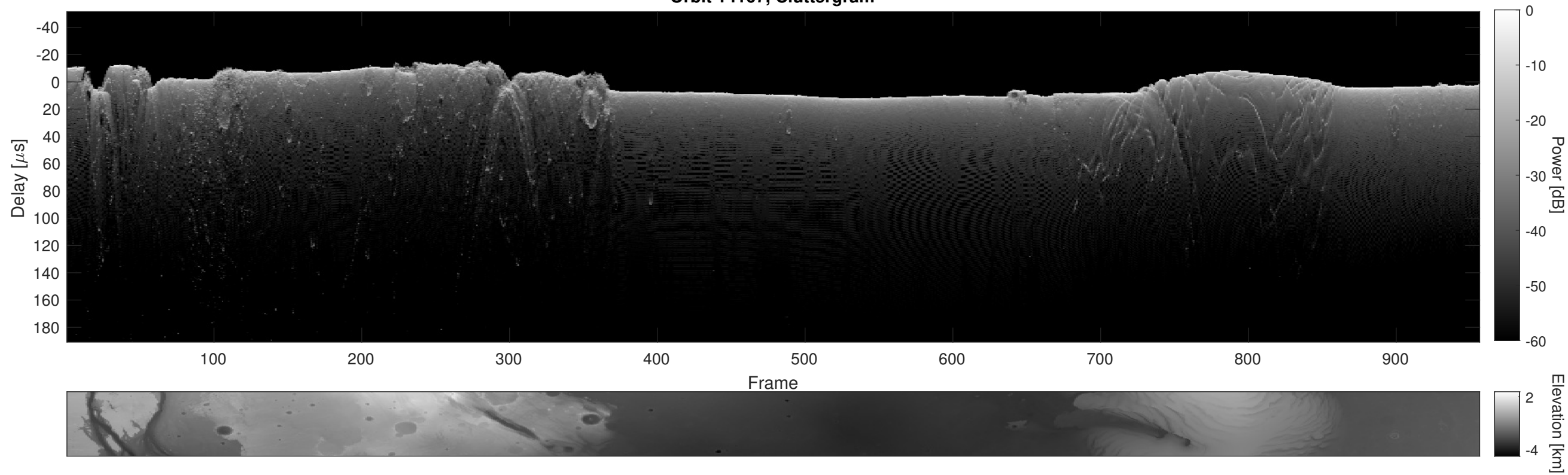
Orbit 14167, Cluttergram
