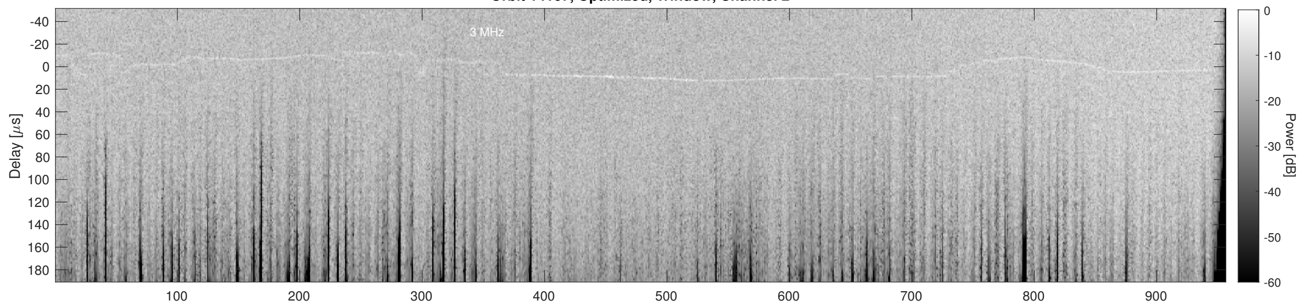
Orbit 14167, Cluttergram
