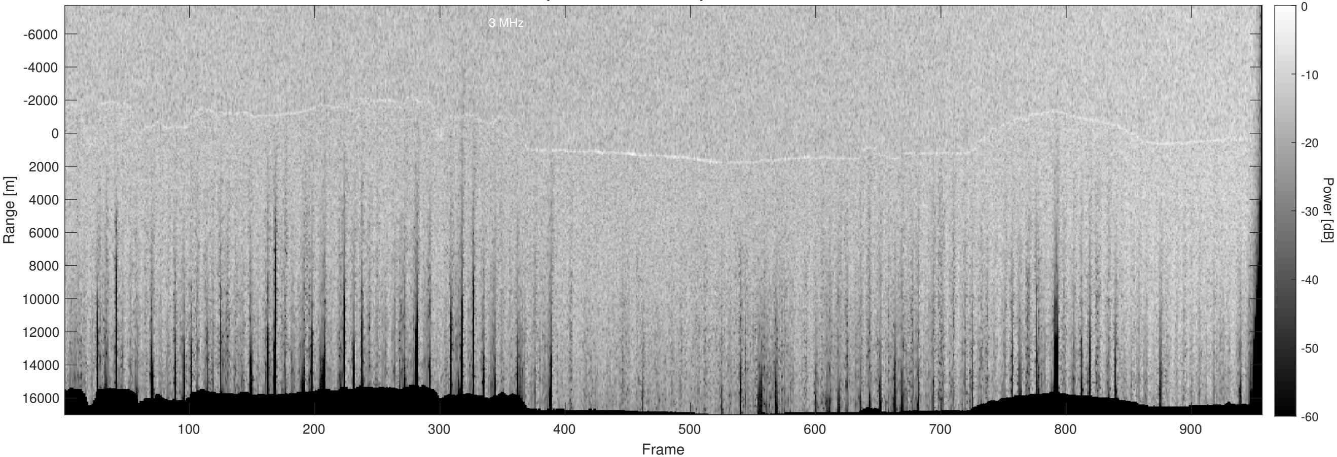
Orbit 14167, Optimized, Window, Depth-Corrected, Channel 2
