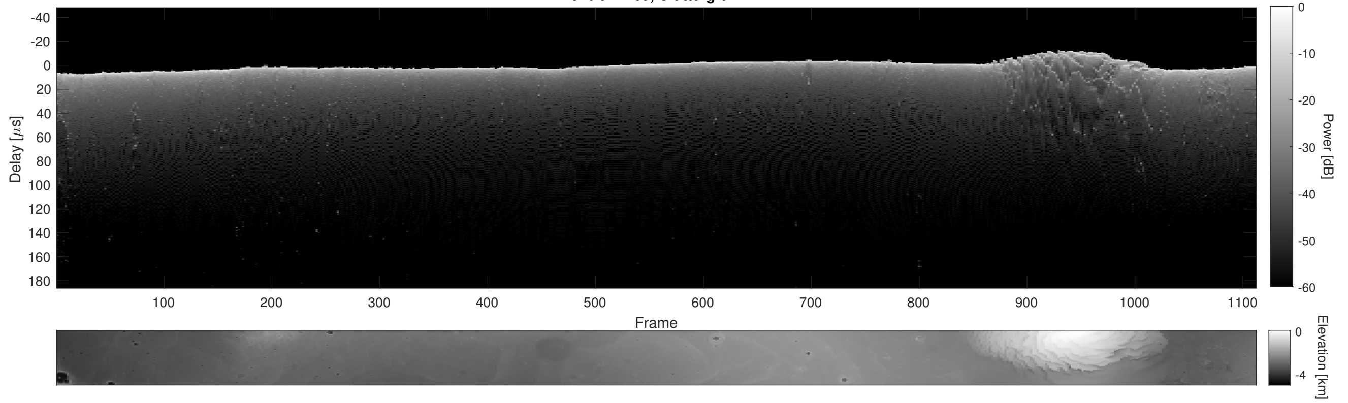
Orbit 14169, Cluttergram
