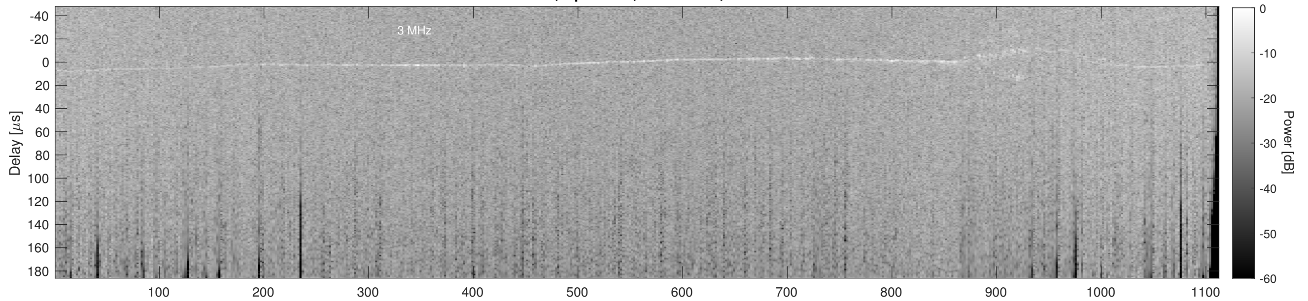
Orbit 14169, Cluttergram
