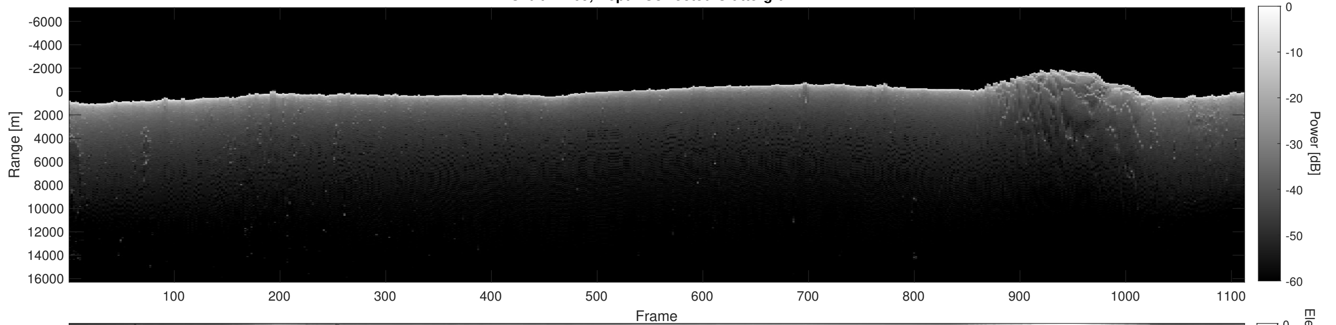
Orbit 14169, Depth-Corrected Cluttergram
