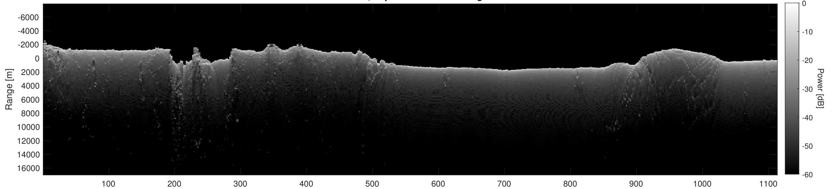
Orbit 14174, Depth-Corrected Cluttergram
