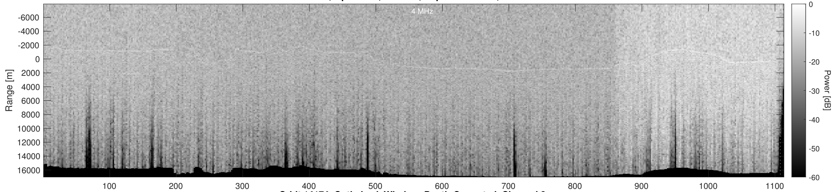
Orbit 14174, Optimized, Window, Depth-Corrected, Channel 2
