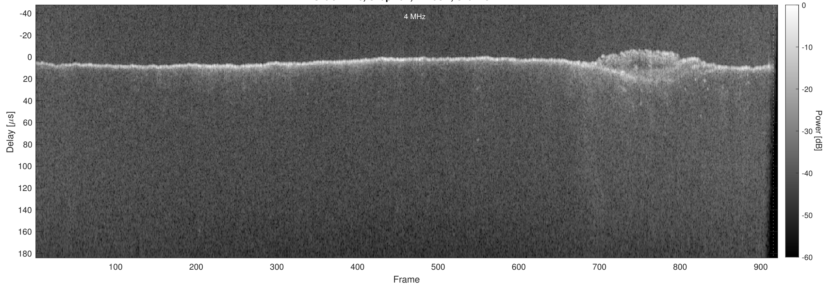
Orbit 14176, Chapman, Window, Channel 2
