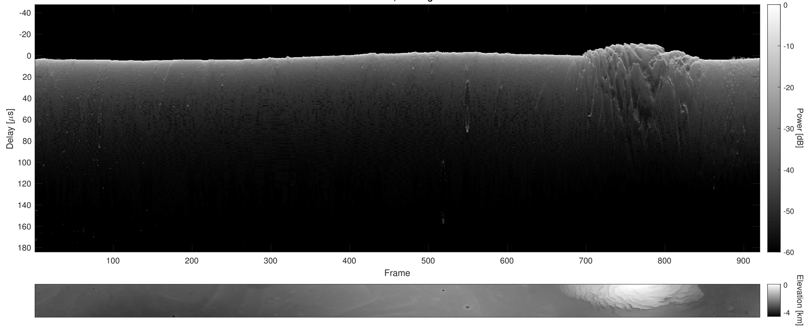
Orbit 14176, Cluttergram
