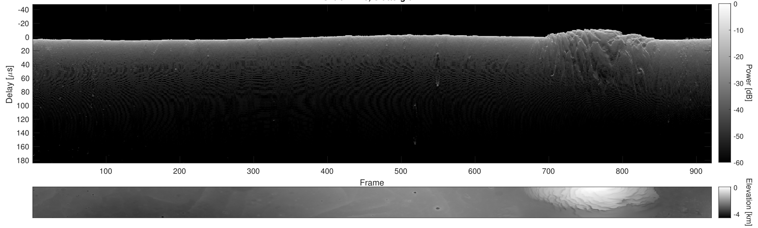
Orbit 14176, Cluttergram
