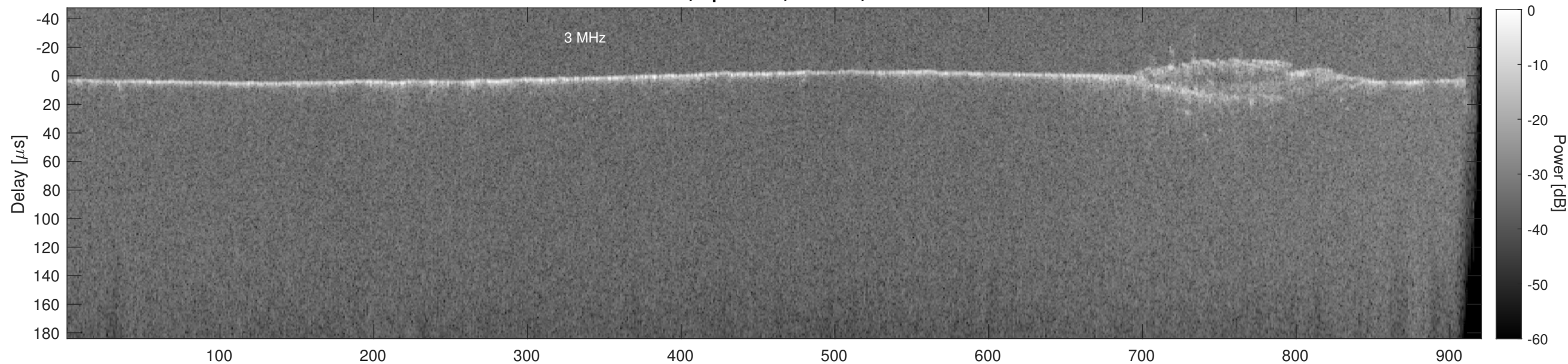
Orbit 14176, Cluttergram
