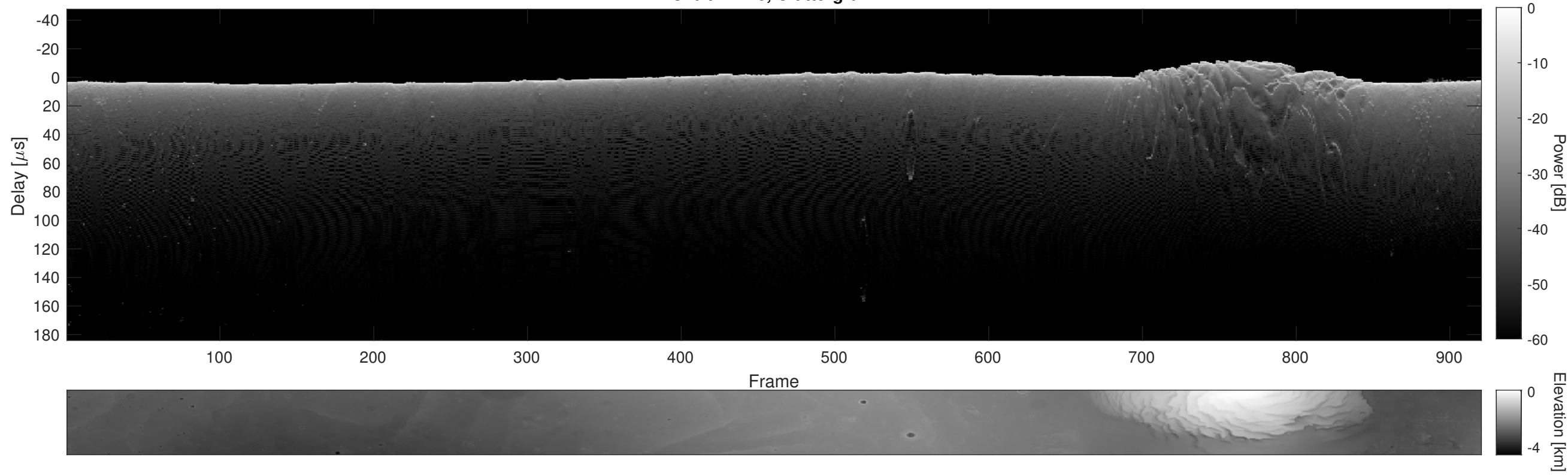
Orbit 14176, Cluttergram
