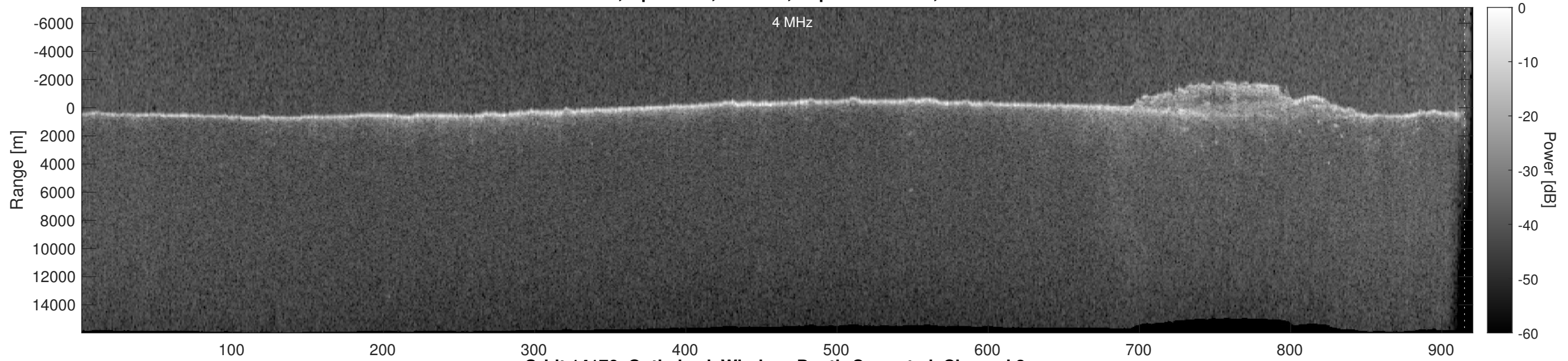
Orbit 14176, Optimized, Window, Depth-Corrected, Channel 2
