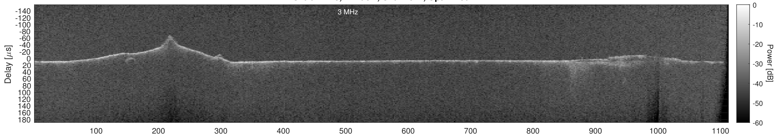
Orbit 14179, Cluttergram
