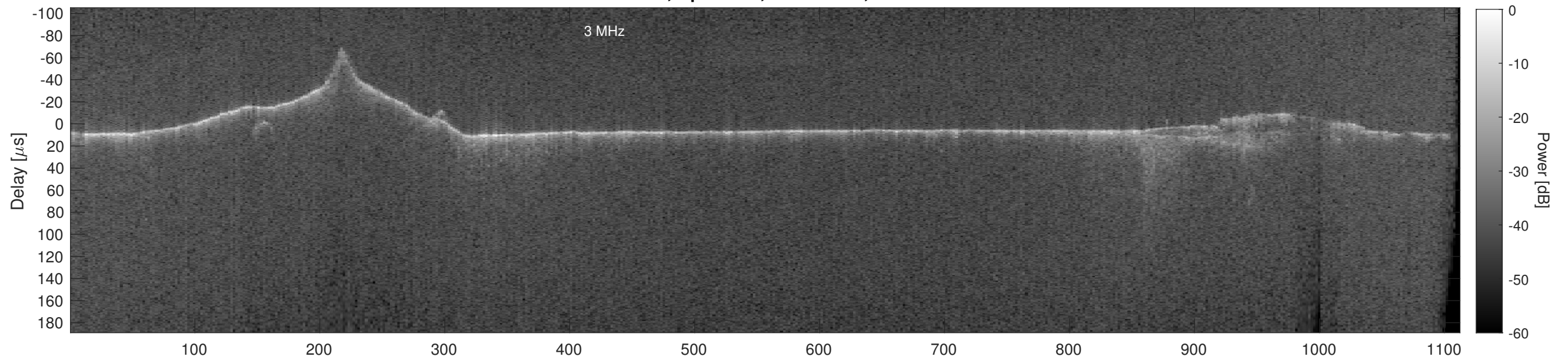
Orbit 14179, Cluttergram
